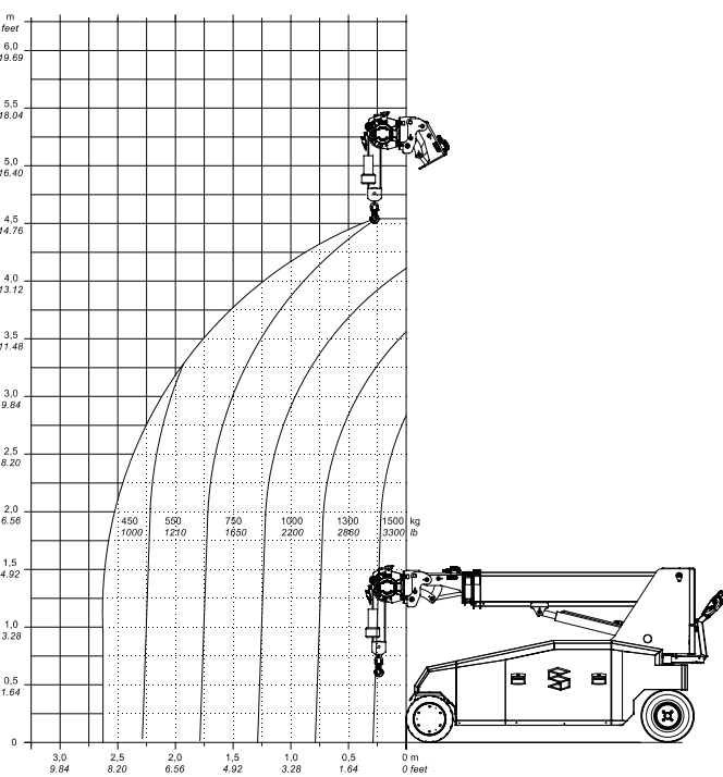
SLX 2000 HYDRAULIC WINCH
