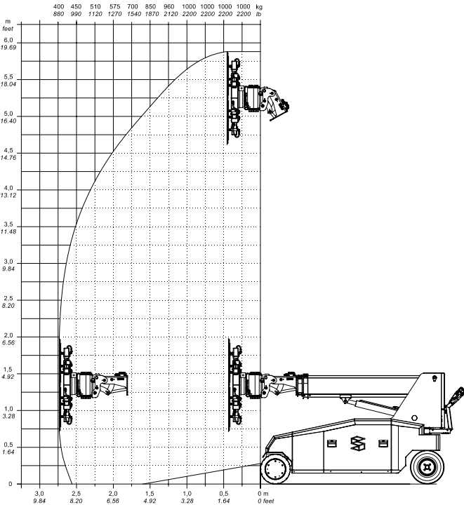
SLX 2000 VACUUM YOKE
