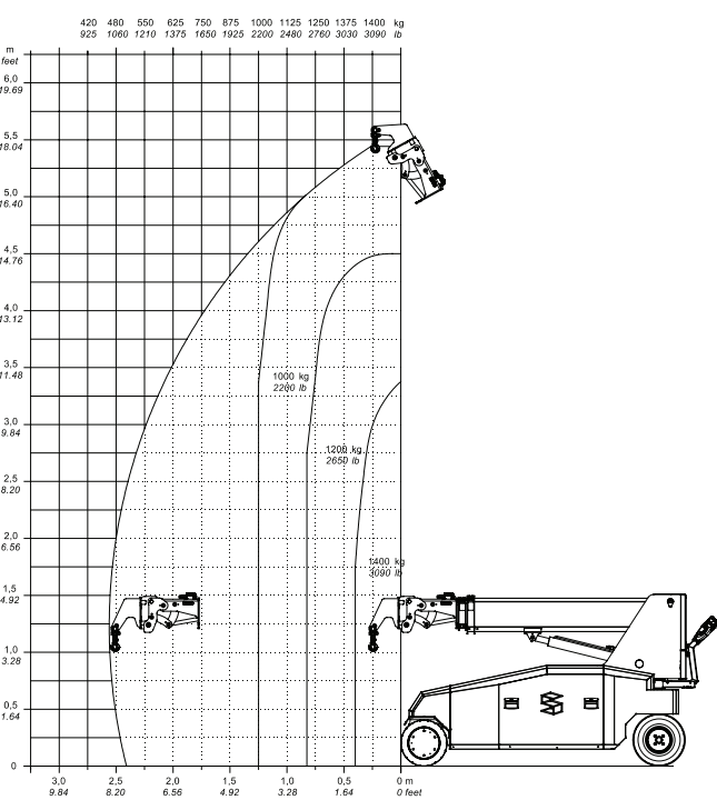
SLX 2000 LIFTING HOOK
