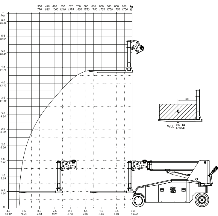
SLX 2000 PALLET FORKS
